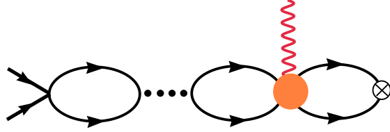
Figure 16: An additional graph at NLO including an insertion of the L_1 operator. From ref. [19], courtesy of M. Savage.
