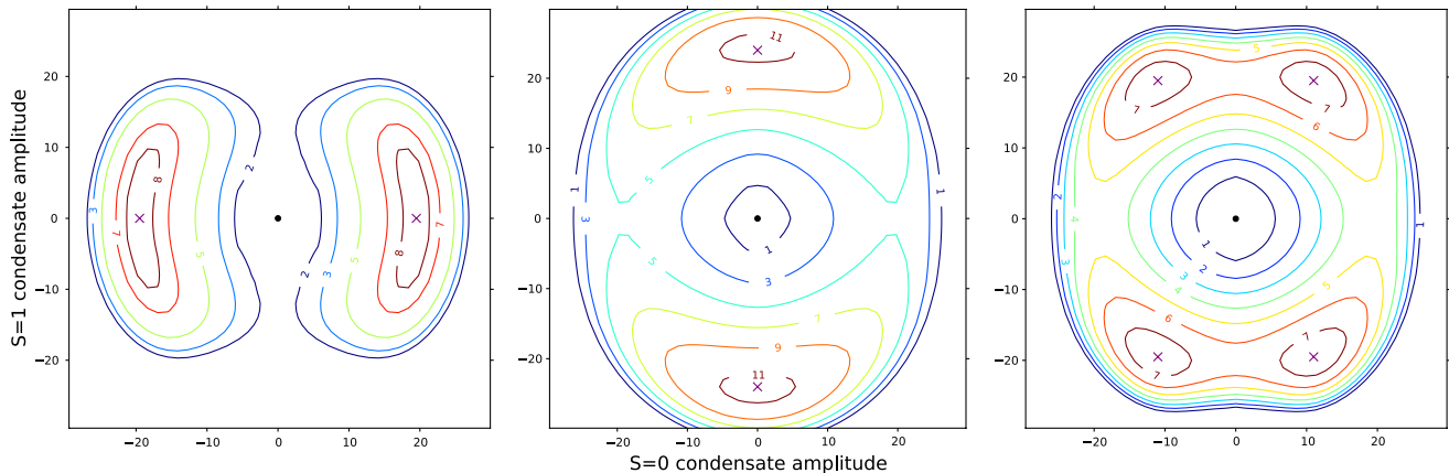
FIG. 2 (color online). Contour plots of the correlation energy in three different A = 132 nuclei as a function of the amplitudes of selected spin-singlet and spin-triplet condensates. Left panel: ^{132}_{60}\text{Nd} , mainly spin-singlet pairing, as is common in most nuclei studied to date; middle panel: ^{132}_{66}\text{Dy} , mainly spin-triplet pairing, similarly to what was introduced in Ref. [3]; right panel: ^{132}_{64}\text{Gd} , mixed-spin pairing exemplifying a qualitatively new feature, namely, the gradual crossover from spin-singlet to spin-triplet pairing. The numbers show correlation energies in MeV. In all three cases, each peak is marked by an X.
