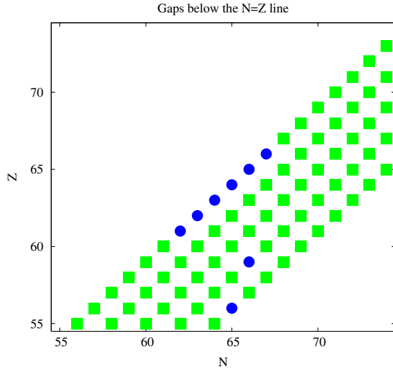
FIG. 3 (color online). Small and large pairing gaps [Eq. (6)] for nuclei near the spin-triplet pairing region. Blue circles: \Delta_0^{(3)}(n) < 0.4 MeV; green squares: \Delta_0^{(3)}(n) > 0.4 MeV.
