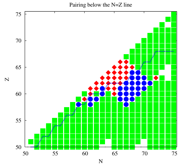
FIG. 1 (color online). Chart of nuclides with Z \leq N for neutron numbers from 50 to 75. Blank squares denote nuclei that exhibit practically no pairing ( E_{\text{corr}} < 0.5 MeV), green squares signify the case where the pairing condensate is mostly spin-singlet, red diamonds are used for the nuclei that exhibit spin-triplet pairing, while blue circles denote nuclei for which the pairing is a mixture of spin-singlet and spin-triplet. The blue dashed line is the proton-drip line from Ref. [16].
