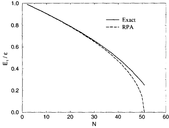
Fig. 1. Energy of the one phonon state as a function of the number of particle. The solid line is the exact solution of the Lipkin model, whilst the dashed line is obtained in the RPA. The strength of the interaction V/\epsilon is set to be 0.01.
