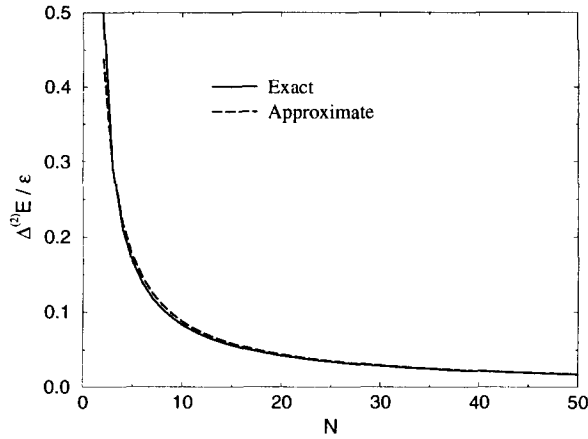
Fig. 3. Anharmonicity of the double phonon state as a function of the number of particle for \chi = 0.25 . The dashed line is an approximate solution given by Eq. (42), while the solid line is obtained by numerically diagonalising the Hamiltonian.
