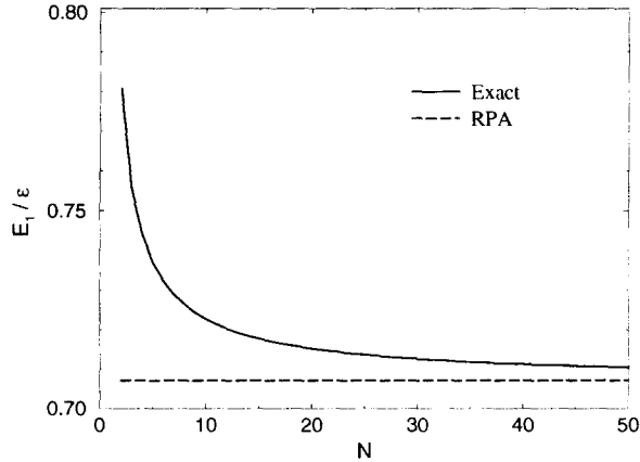
Fig. 2. Same as Fig. 1, but for a fixed \chi parameter, which is set to be 0.25.
