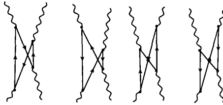
Fig. 4. The diagrams of order 1/N contributing to the anharmonicity of the double phonon state for the Hamiltonian (1). The wavy lines represent phonon propagations, while the particles and the holes are depicted by the allowed lines.
