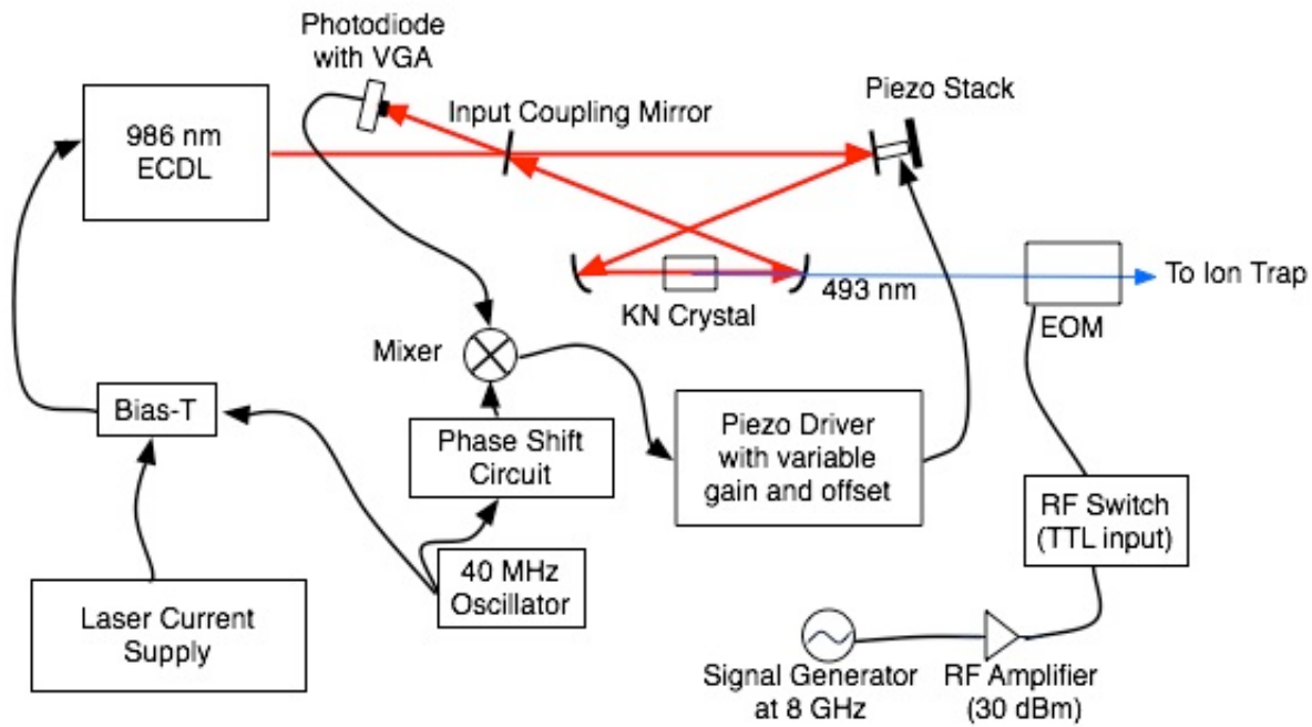
Figure 1: Diagram of entire blue cooling laser apparatus
