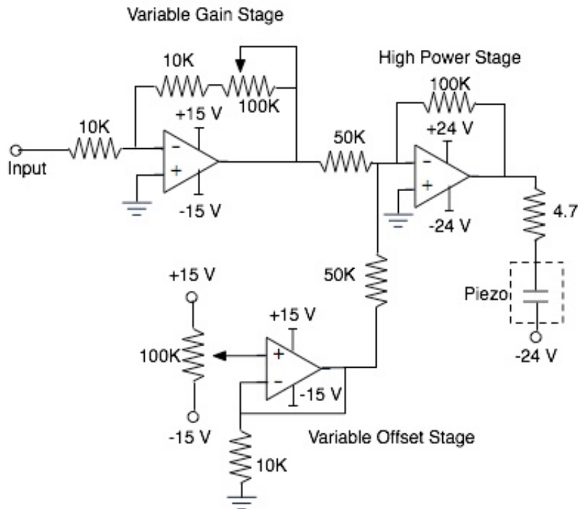
Figure 2: Piezo driver circuit diagram
