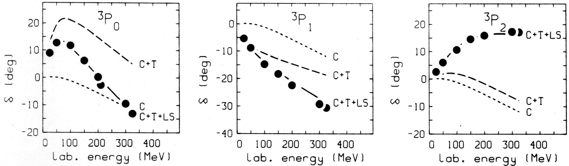
Fig. 3.3. NN phase shifts in triplet P waves. Shown are predictions using a central (C) central plus tensor (C+T) and also including spin-orbit interactions (C+T+LS).
