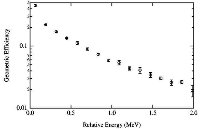
FIG. 7. Geometric efficiency for detecting protons and ^7\text{Be} fragments in coincidence from the Coulomb dissociation of 83 MeV/nucleon ^8\text{B} with impact parameters \geq 30 fm. The relative errors shown are statistical uncertainties from the simulation and theoretical uncertainties from the size of the E2 component, added in quadrature.
