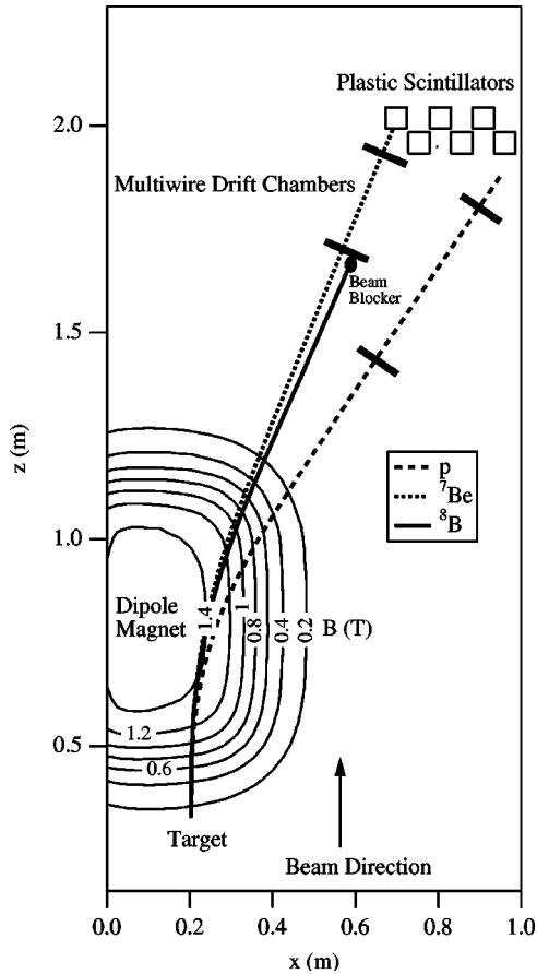
FIG. 4. Schematic view of the experimental setup for the exclusive measurement showing the detectors, typical trajectories, and contours of constant magnetic field produced by the dipole magnet.
