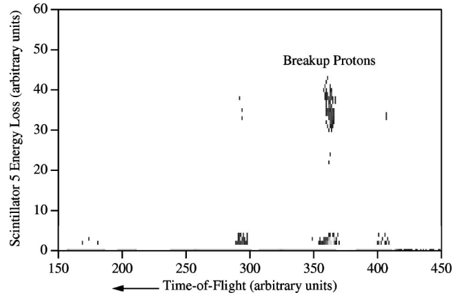
FIG. 5. Typical proton scintillator bar energy loss versus time-of-flight spectrum. The events with small scintillator signals represent crosstalk from adjacent scintillator bars.
