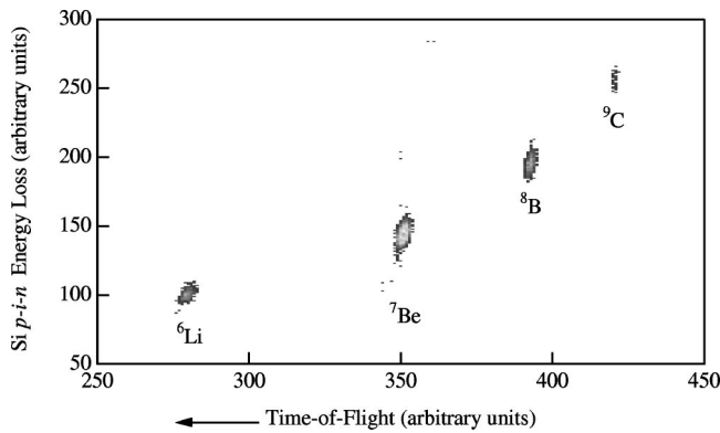
FIG. 2. Typical Si p-i-n diode versus time-of-flight spectrum illustrating the secondary beam composition.
