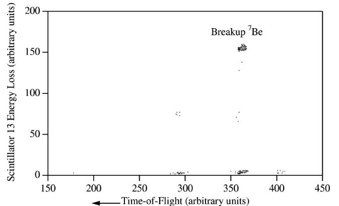
FIG. 6. Typical {}^7\text{Be} scintillator bar energy loss versus time-of-flight spectrum. The events with small scintillator signals are due to light produced in adjacent scintillator bars.
