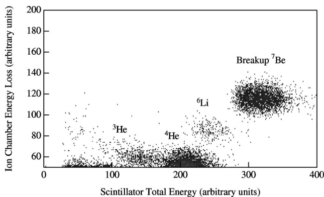
FIG. 3. Typical ionization chamber energy loss versus stopping scintillator total energy spectrum.
