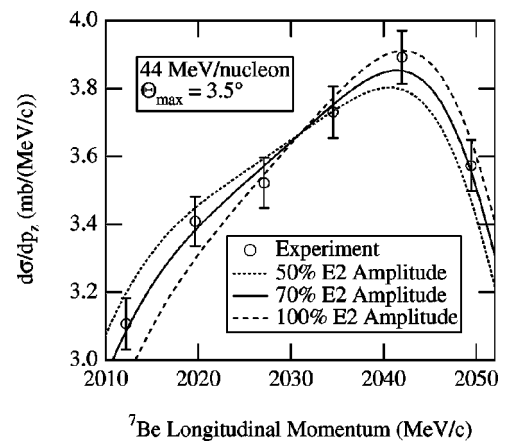
FIG. 14. Central region of the 3.5^\circ angle cut of the {}^7\text{Be} longitudinal momentum distribution from the breakup of 44 MeV/nucleon {}^8\text{B} on Pb. The curves are calculations performed with different E2 matrix elements, expressed in terms of the E2 amplitude of the model of [25], normalized to the center of the distribution.
