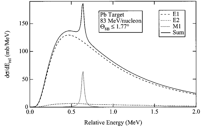
FIG. 15. Contributions of E1 , E2 , and M1 transitions to the cross section for the Coulomb dissociation of 83 MeV/nucleon ^8\text{B} on Pb with ^8\text{B} scattering angles \leq 1.77^\circ in first-order perturbation theory. The M1 cross section is calculated by folding the M1 S factor measured in Ref. [8] with the virtual photon spectrum. The E1 and E2 cross sections are calculated using the model of Ref. [25], scaling the E2 matrix elements by the factor 0.7 required to reproduce the measured ^7\text{Be} longitudinal momentum distributions.
