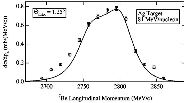
FIG. 11. Laboratory frame longitudinal momentum distribution of {}^7\text{Be} fragments with maximum scattering angles of 1.25^\circ emitted in the Coulomb dissociation of 81 MeV/nucleon {}^8\text{B} on Ag. The curve is a first-order perturbation theory calculation convoluted with the experimental resolution.
