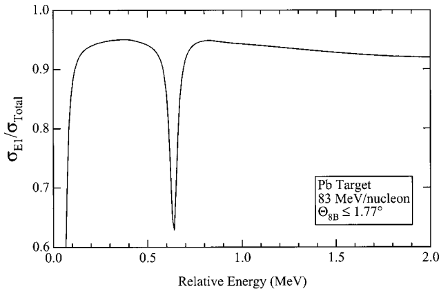
FIG. 16. Fraction of the calculated cross section for the Coulomb dissociation of 83 MeV/nucleon ^8\text{B} on Pb with ^8\text{B} scattering angles \leq 1.77^\circ ( b \geq 30 fm) accounted for by E1 transitions in first-order perturbation theory. As the energy falls below 130 keV, E2 transitions become increasingly important.
