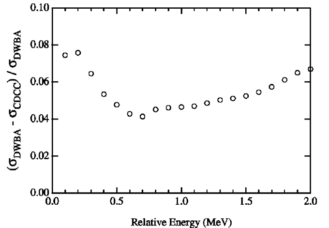
FIG. 18. Difference between the cross section for Coulomb breakup of 83 MeV/nucleon ^8\text{B} on Pb for ^8\text{B} scattering angles of 1.77^\circ and less predicted by DWBA (first-order) and CDCC (all orders) calculations using the same structure model, expressed as a fraction of the DWBA prediction. Only Coulomb matrix elements were included in these calculations. No significant energy dependence of the higher-order electromagnetic effects is evident.
