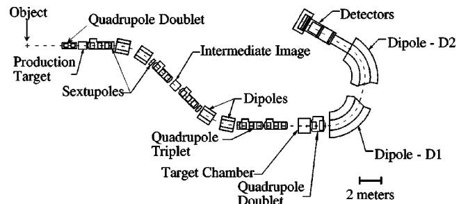
FIG. 1. Schematic view of the S800 spectrometer at the NSCL.
