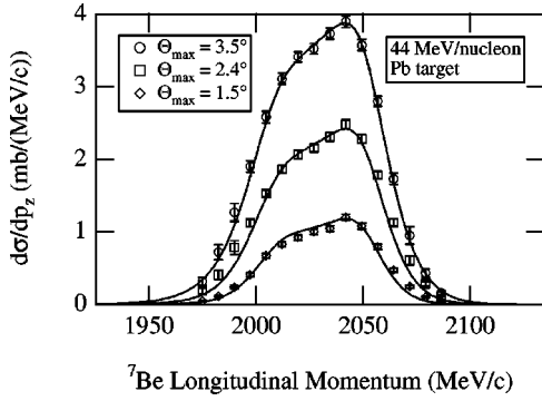
FIG. 8. Measured longitudinal momentum distributions of {}^7\text{Be} fragments from the Coulomb dissociation of 44 MeV/nucleon {}^8\text{B} on Pb with several maximum {}^7\text{Be} scattering angle cuts. Also shown are first-order perturbation theory calculations convoluted with the experimental resolution. See the text for details.
