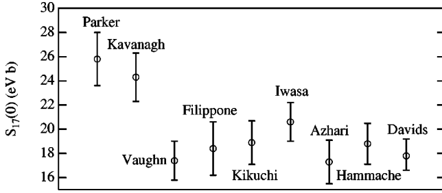
FIG. 19. Inferred zero-energy astrophysical S factors for the {}^7\text{Be}(p, \gamma){}^8\text{B} reaction from selected direct and indirect measurements. The data are from Refs. [4–6,8,16,17,46,10], and the present work.
