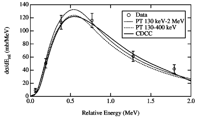
FIG. 17. Measured differential cross section for the Coulomb dissociation of 83 MeV/nucleon ^8\text{B} on Pb with ^8\text{B} scattering angles \leq 1.77^\circ . Only relative errors are shown. Also depicted are continuum-discretized coupled channels and two first-order perturbation theory calculations, convoluted with the experimental resolution. The point at 64 keV has been excluded from the fits because E2 transitions are dominant at this energy.
