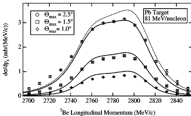
FIG. 12. Laboratory frame longitudinal momentum distribution of {}^7\text{Be} fragments emitted in the Coulomb dissociation of 81 MeV/nucleon {}^8\text{B} on Pb with maximum scattering angles of 2.5^\circ , 1.5^\circ , and 1.0^\circ . The solid curves are continuum-discretized coupled channels calculations that include both Coulomb and nuclear interactions, convoluted with the experimental resolution. The dashed curve is a DWBA calculation for \Theta_{\text{max}} = 2.5^\circ .
