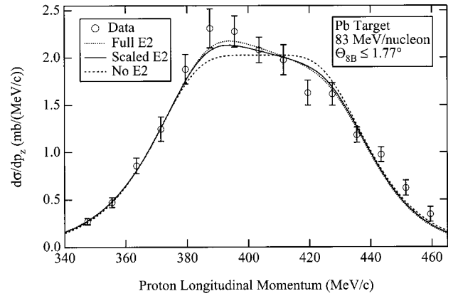
FIG. 13. Measured longitudinal momentum distribution of protons from the Coulomb dissociation of 83 MeV/nucleon {}^8\text{B} on Pb with {}^8\text{B} scattering angles \leq 1.77^\circ . Only relative errors are shown. Also depicted are first-order perturbation theory calculations with different E2 strengths, convoluted with the experimental resolution.
