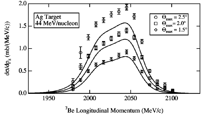
FIG. 9. Laboratory frame longitudinal momentum distributions of {}^7\text{Be} fragments with maximum scattering angles of 2.5^\circ , 2.0^\circ , and 1.5^\circ emitted in the breakup of 44 MeV/nucleon {}^8\text{B} on Ag. The solid curves represent perturbative Coulomb dissociation calculations convoluted with the experimental resolution.
