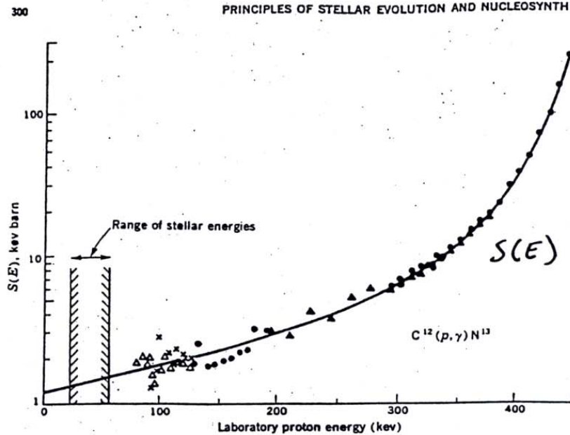
Fig. 4-5 The cross-section factor S(E) for the radiative capture of protons by \text{C}^{12} . The differing types of data points represent five different experiments performed at different times and laboratories by the workers indicated. Detailed references and discussion may be found in D. F. Hebbard and J. L. Vogl, Nucl. Phys. , 21 :652 (1960). This curve is more readily extrapolated than the one in Fig. 4-4.
