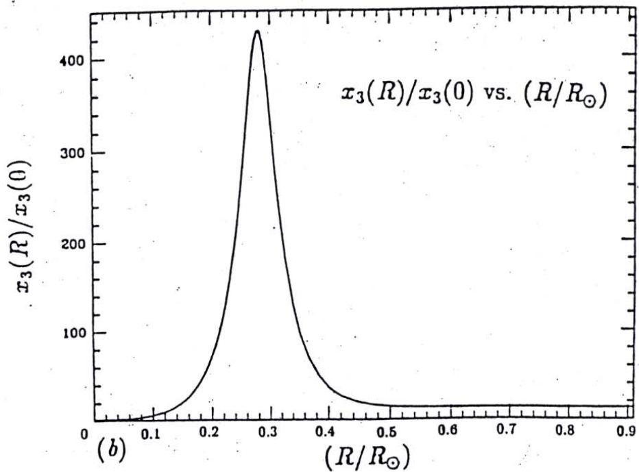
Figure 4.2 Composition fractions as a function of radius Figure 4.2a shows the logarithm of the hydrogen, X_1 , and helium, X_4 , mass fractions as a function of position in the standard solar model. Figure 4.2b illustrates the dependence of the ^3\text{He} abundance upon position [from Bahcall and Ulrich (1988)].
