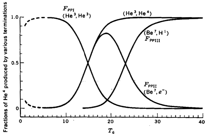
Figure 3.14: Fraction of {}^4\text{He} produced by the ppI, ppII and ppIII chains, as a function of temperature. The chains are assumed to be in equilibrium, and it was assumed that Y = X . Figure from Clayton (1968).
