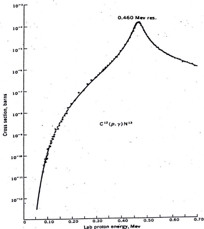
Fig. 4-4 The measured cross section for the reaction C^{12}(p, \gamma)N^{13} as a function of laboratory proton energy. A four-parameter theoretical curve has been fitted to the experimental points. An extrapolation to E_p = 0.025 Mev, which is an interesting energy for this reaction in astrophysics, appears treacherous. (Courtesy of W. A. Fowler and J. L. Vogt.)
