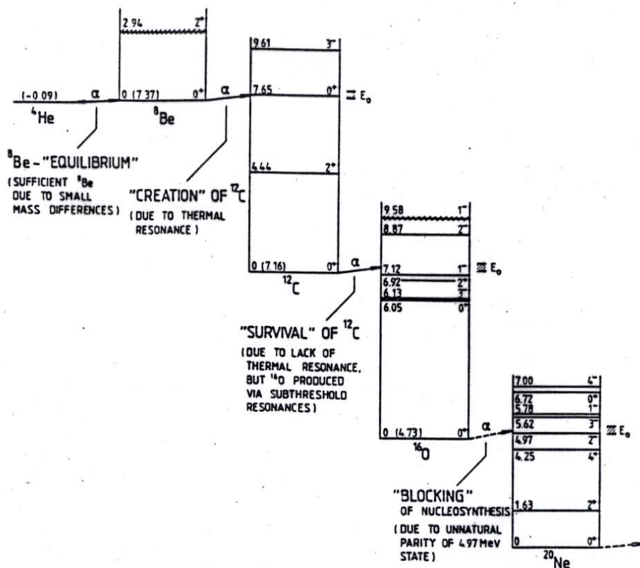
FIGURE 7.15. Shown in perspective are the level schemes of the nuclei involved in the helium-burning reactions in red giants. It is only through a number of fortuitous nuclear properties as well as parity and isospin conservation laws that carbon and oxygen, the essential elements for life as we know it, are the major products of nucleosynthesis in red giants.
