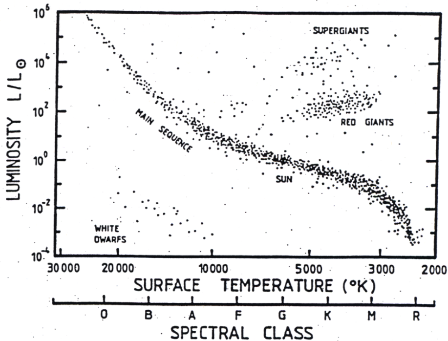
FIGURE 1.24. The Hertzsprung-Russell (H-R) diagram is shown schematically. Most of the stars (including the sun) are grouped along a band called the main sequence. As one goes from the upper left-hand corner to the lower right-hand corner along the main sequence, the temperature, mass, size, and luminosity decrease, while the mean density increases. The diagram represents a snapshot in the history of the stars' lives. The wide variety of stellar masses and the resulting variety of evolutionary tracks reflect the diversity of stellar objects. Note that only a small fraction of low-mass main-sequence stars is shown.
